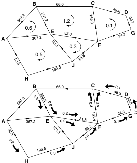
Figure 1.14 Network adjustment. (a) The 1.2 unit misclosure in loop BCFE suggests a large error in either the 'unsupported' link BC or in BE, the only link shared with another loop with a large misclosure. (b) Adjustments made on the assumption that BC was checked and found to be correct but that no other checks could be made.
