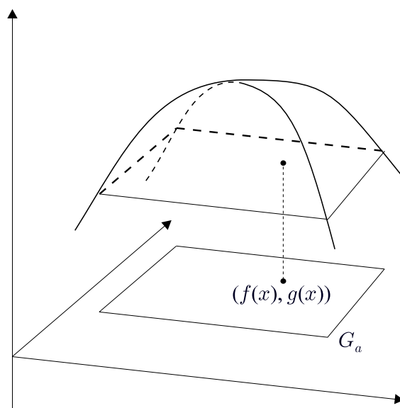
Figure 3.3 The sets G_a
