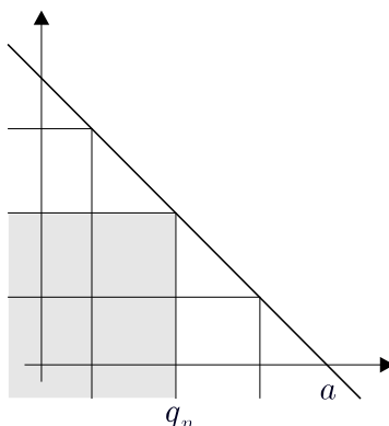
Figure 3.2 Boxes
