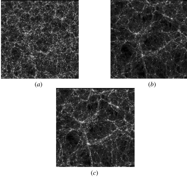
Figure 15.16. (a) Standard CDM (standard CDM \rightarrow \Omega_{\text{matter}} = 1.0, \Omega_{\Lambda} = 0.0, H_0 = 50 \text{ kps/Mpc} ), (b) open CDM (open CDM \rightarrow \Omega_{\text{matter}} = 0.3, \Omega_{\Lambda} = 0.0, H_0 = 70 \text{ kps/Mpc} ), (c) lambda CDM (lambda CDM \rightarrow \Omega_{\text{matter}} = 0.3, \Omega_{\Lambda} = 0.7, H_0 = 70 \text{ kps/Mpc} ). Computer graphics produced by a program designed to simulate the evolution of matter under gravity from the early universe up to the present time. The brighter the spot, the denser the clustering of matter is at that point. The figure on the left is generated from a model that contains cold dark matter and with a universe that has a cosmological constant. That on the right is the same, but without the cosmological constant. (These images are courtesy of the ‘Virgo consortium for cosmological simulations’, a collaboration between the Universities of Durham, Sussex, Cambridge and Edinburgh in the UK, the Max Planck Institute for Astrophysics in Germany and the MacMaster University in Canada. The members of the consortium are H Couchman, G Efstathiou, C S Frenk (Principal Investigator), A Jenkins, J Peacock, F Pearce, V Springel, P Thomas, S White and N Yoshida. The work of the Virgo consortium is carried out on a Cray-T3Es at the Max-Planck Rechen Zentrum in Garching and the Edinburgh Parallel Computing Centre.)
