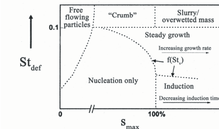
Figure 11: Modified granule growth regime map (Iveson et al., 2001b).
