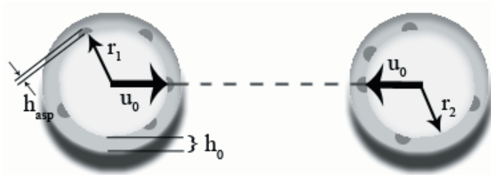
Figure 7: Principles of the original Ennis et al. agglomeration model.
