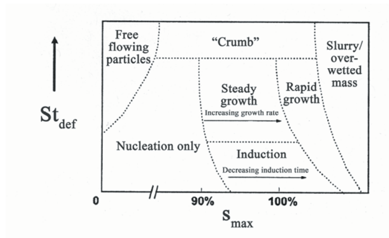
Figure 10: Granule growth regime map (Iveson & Litster, 1998).
