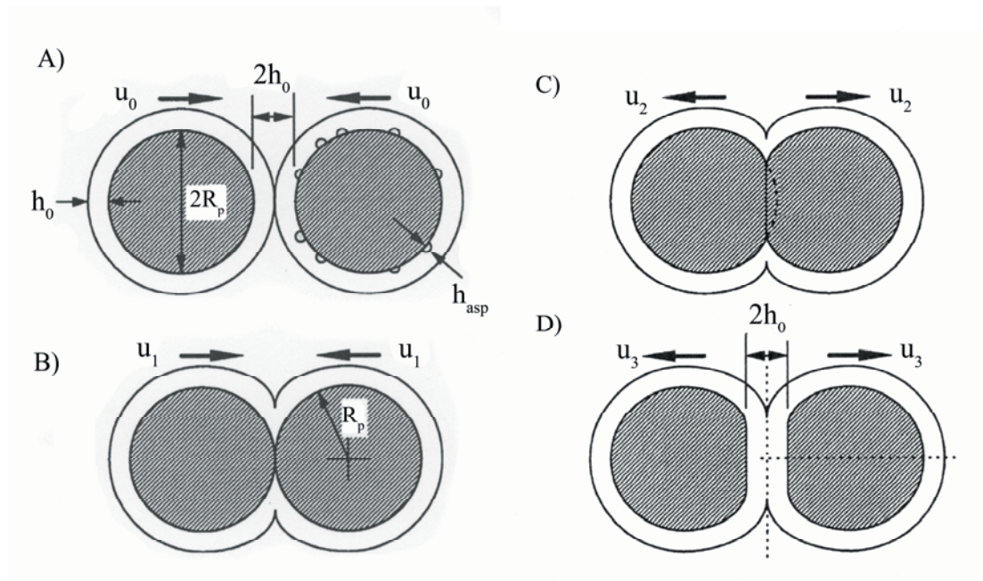
Figure 8: Stages in the agglomeration process of deformable primary particles.
