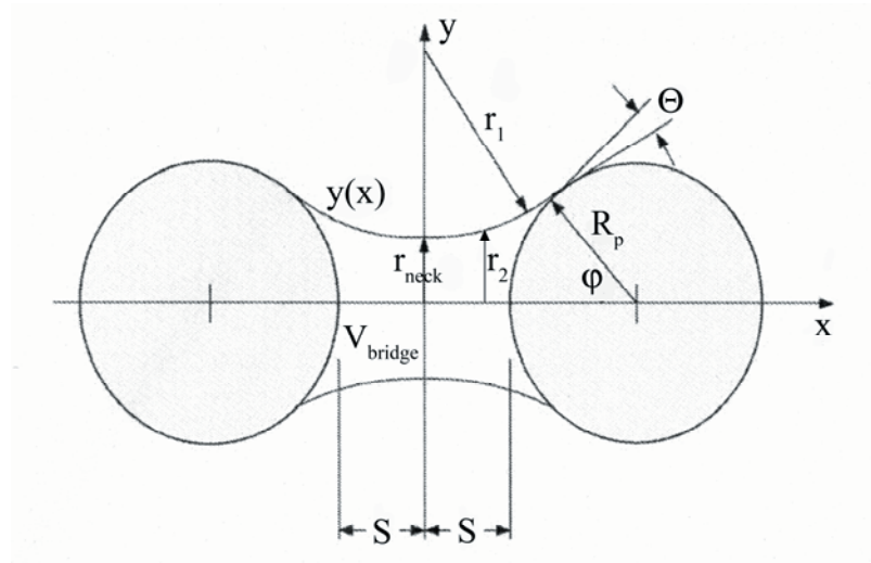
Figure 4: Formal bonding schematic of an agglomerate.
