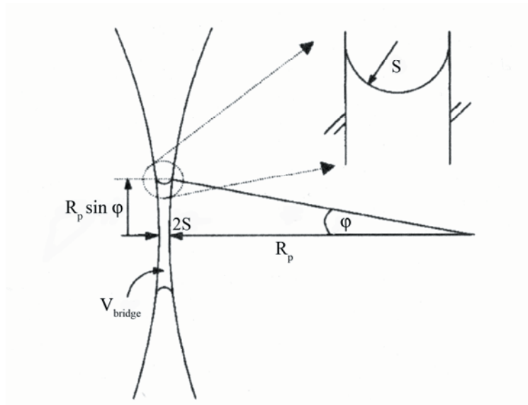
Figure 5: Liquid bridge bonding two primary particles.
