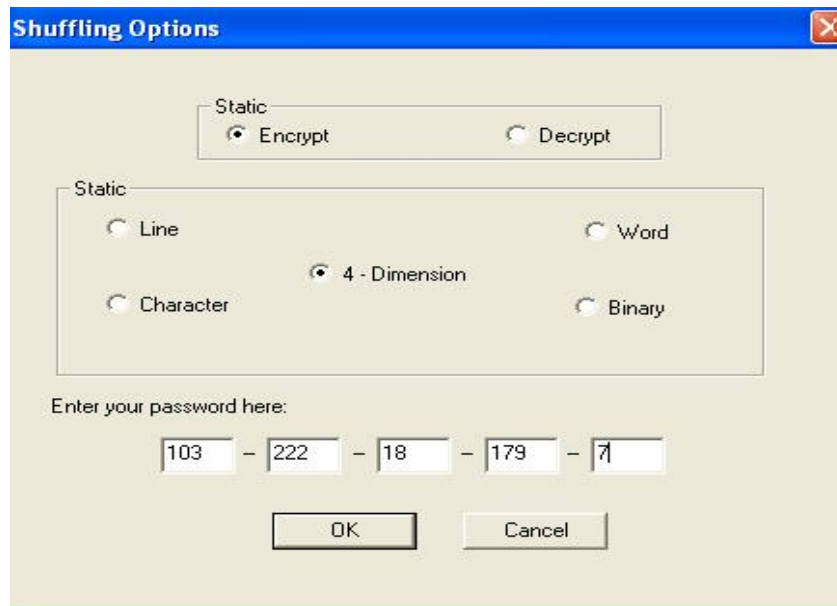
Fig (1): Selection of dimension and secret key management.
