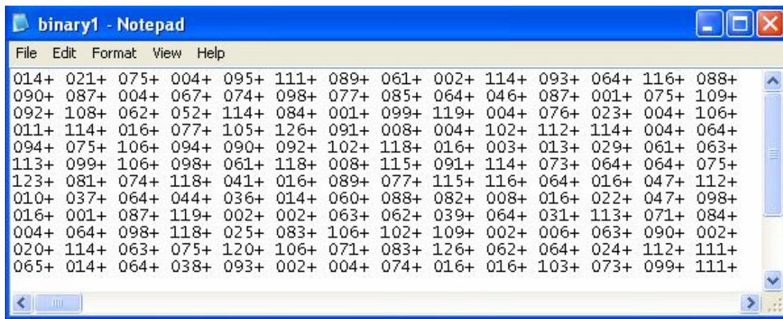
Fig (6): Applying Binary encryption to the text of Fig(2).
