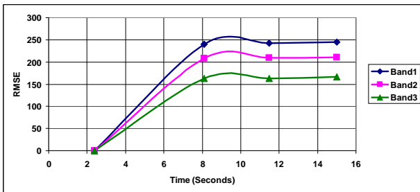
Figure 16. Sample 3 RMSE.
