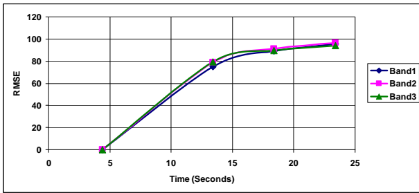
Figure 14. Samples 1 RMSE.
