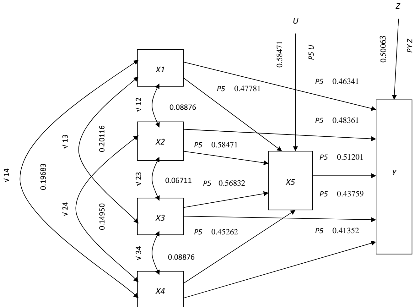
Figure 3: Path Diagram for the Direct, Indirect, and Total Effects of IT Governance and AIS on the Usefulness of Accounting Information
