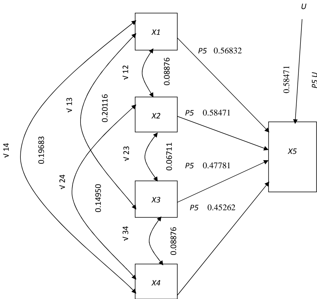
Figure 2: Path Diagram for the Direct and Total Effects of IT Governance on the AIS
