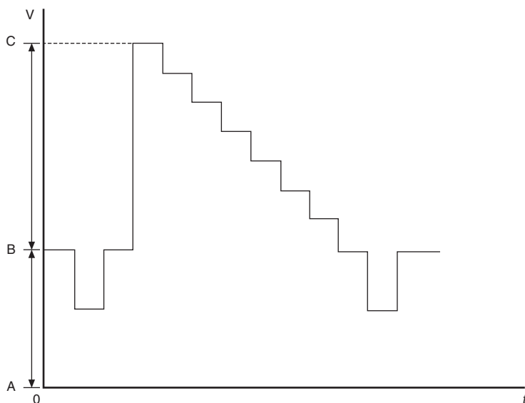
Figure 7.3 Sync separator action
