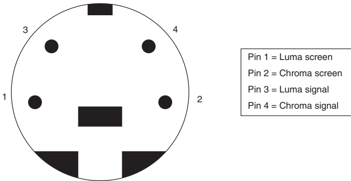
Figure 5.19 S-VHS connector pin configuration
