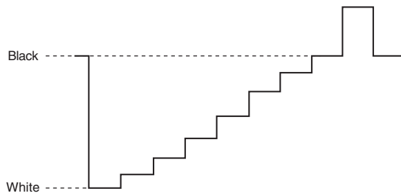
Figure 6.13 Staircase signal with gamma correction (exaggerated)
