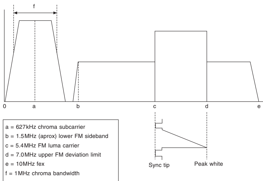
Figure 8.8 S-VHS signal spectrum
