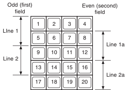
Figure 6.2 Method of adding CCD charge outputs to derive different TV lines for each (interlaced) field
