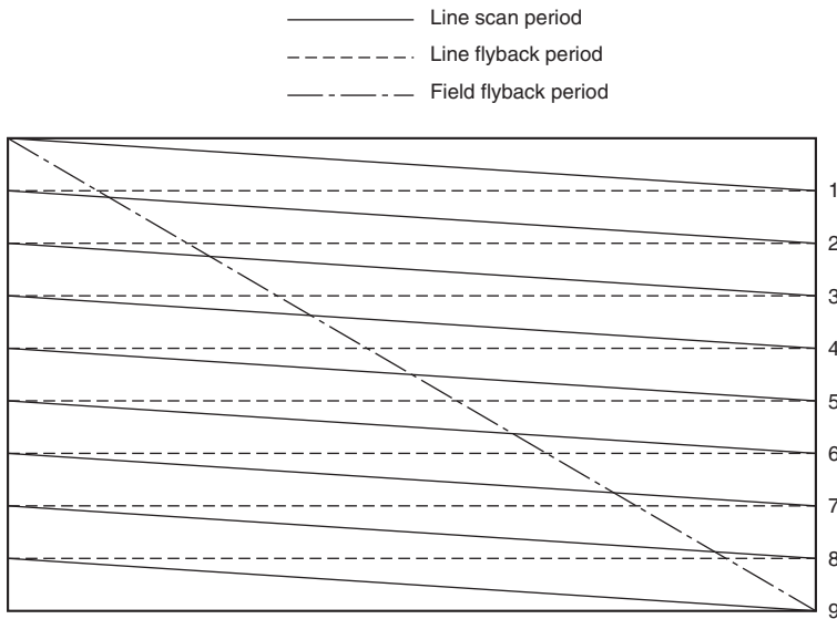
Figure 5.6 Nine line sequentially scanned raster
