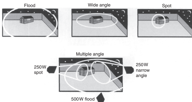
Figure 3.11 In some situations a mixture of lighting distributions is required to provide adequate illumination
