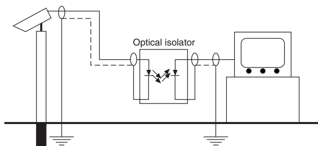
Figure 2.14 Principle of a single channel opto-isolator
