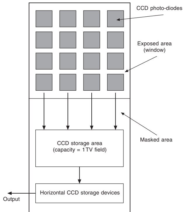
Figure 6.4 Frame transfer CCD chip principle
