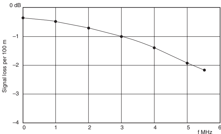
Figure 2.7 Frequency losses in a typical co-axial cable
