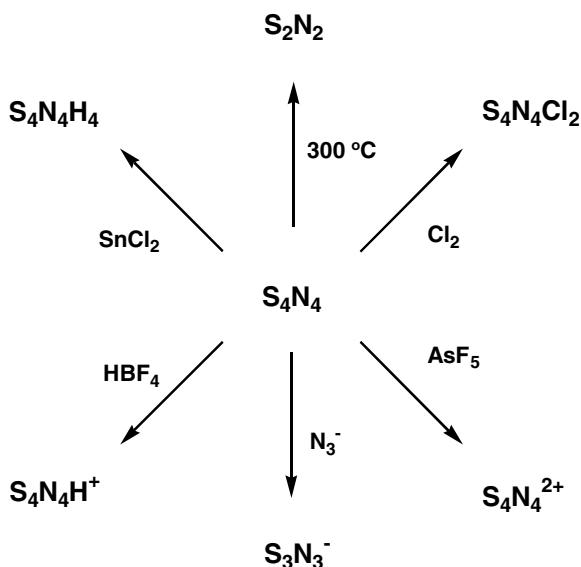
Scheme 5.1 Preparation of S–N rings from \text{S}_4\text{N}_4
