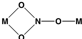
Fig. 1.1 Typical coordination modes for [\text{NS}_3]^- and [\text{NO}_3]^-
