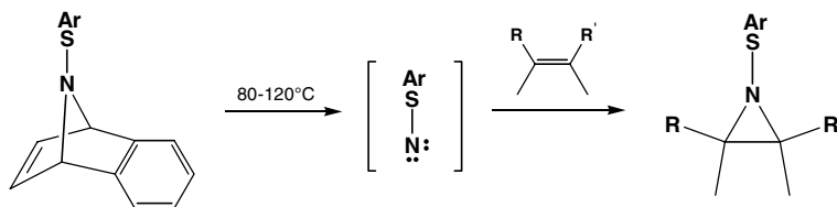
Scheme 10.9 Formation and trapping of an arenesulfonylnitrene (Ar = Ph, 2,4- (\text{NO}_2)_2\text{C}_6\text{H}_3 )
