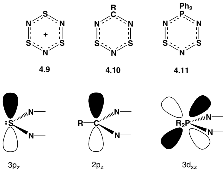
Fig. 4.5 The isolobal groups S^+ , CR and \text{PR}_2
