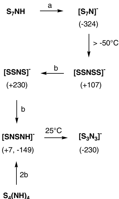
Scheme 5.6 Sulfur–nitrogen anions formed in the deprotonation of \text{S}_7\text{NH} and \text{S}_4\text{N}_4\text{H}_4 ( a = \text{NH}_3(\text{l}) ; b = \text{KNH}_2 ). Nitrogen NMR chemical shifts (in ppm) are given in parentheses [ref. \text{MeNO}_2(\text{l}) ]
