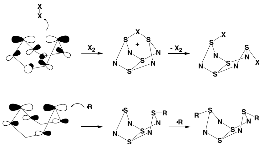
Fig. 4.14 Polar and radical oxidations of S_4N_4
