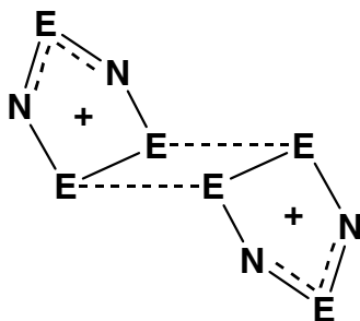
Fig. 4.9 Structure of \text{E}_6\text{N}_4^{2+} ( \text{E} = \text{S}, \text{Se} )
