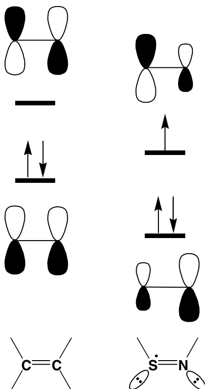
Fig. 4.1 Qualitative comparison of the \pi -molecular orbitals of \text{H}_2\text{C}=\text{CH}_2 and \text{HSNH}
