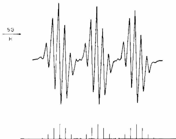
Fig. 3.3 EPR spectrum of [(\text{CF}_3\text{S})_2\text{N}]^\bullet [Reproduced with permission from, J. Am. Chem. Soc. , 105 , 1504 (1983)]
