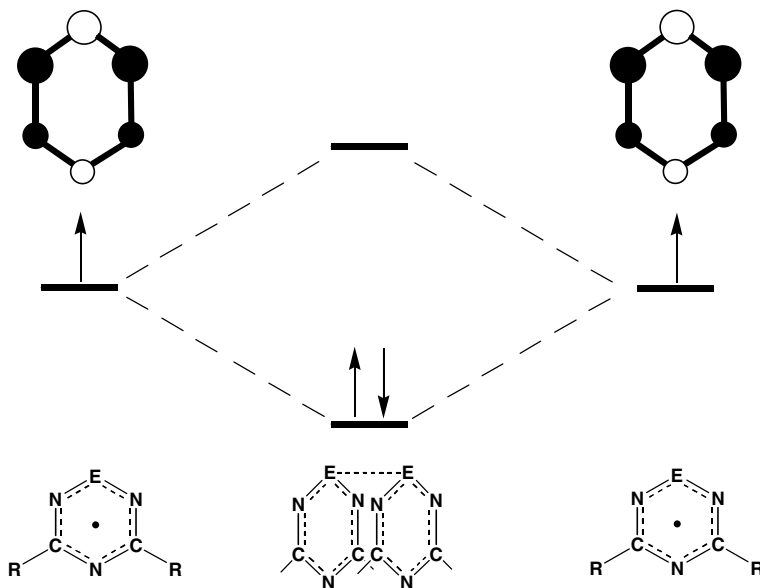
Fig. 4.11 Cofacial overlap of two [(\text{PhC})_2\text{N}_3\text{E}]^\bullet ( \text{E} = \text{S}, \text{Se} ) radicals
