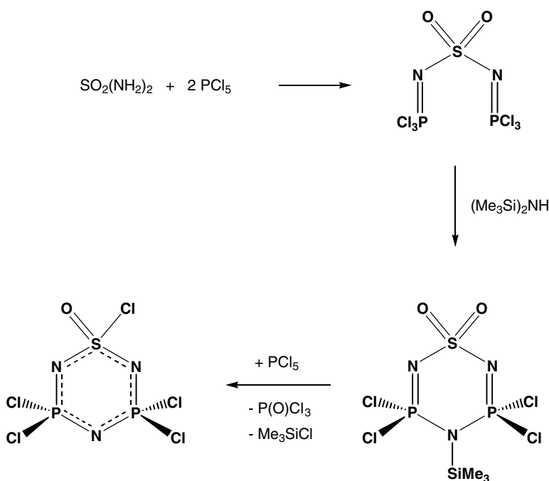
Scheme 13.1 Synthesis of (\text{NPCl}_2)_2[\text{NS}(\text{O})\text{Cl}]
