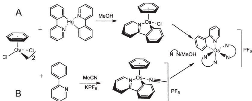
SCHEME 19. Synthetic routes to cyclometalated \text{Os}^{\text{II}} mediators.
