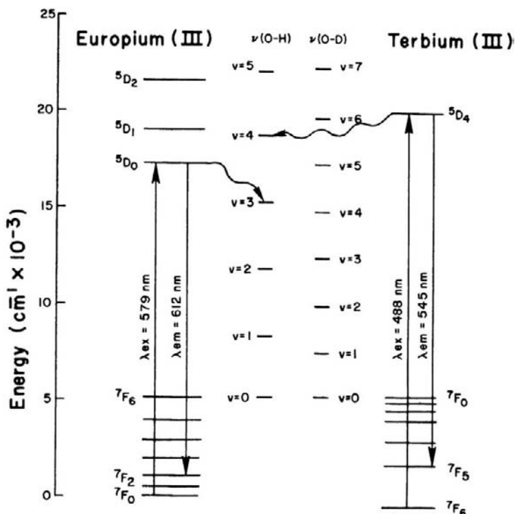
FIG. 3. Deactivation of europium and terbium excited states by energy transfer to O-H and O-D oscillator overtone vibrations. Reprinted with permission from Acc. Chem. Res. 1981, 14, 384-392. Copyright 1981 American Chemical Society.
