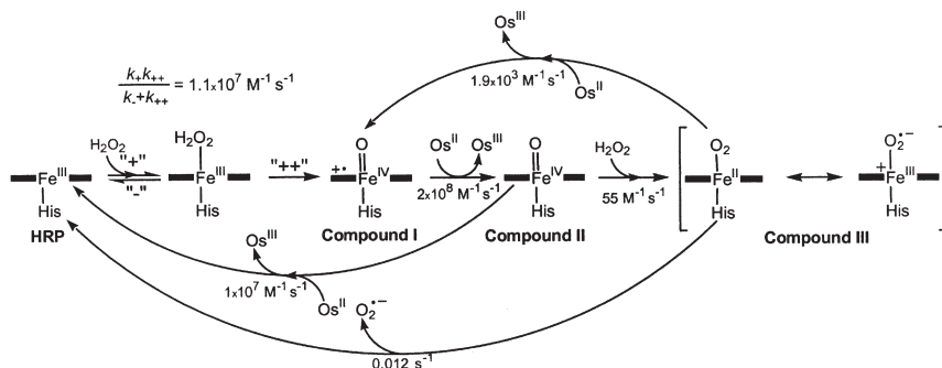
SCHEME 15. Detailed mechanism of HRP catalysis in the system HRP–H 2 O 2 –[Os(bpy) 2 (py)(H 2 O) 2 ] 2+ at pH 7.4 and 20 °C (121).
