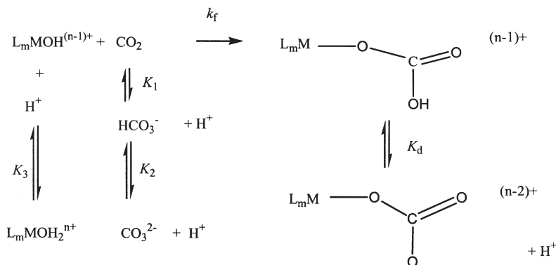
SCHEME 2. CO 2 uptake reaction of [L m MOH] (n-1)+ species.
