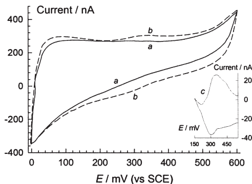
FIG. 12. Cyclic voltammograms of HRP ( a ), Fc-HRP ( b ), and the difference ( a - b ) trace ( c ) in aqueous solution ( [\text{Fc-HRP}] 1.3 \times 10^{-5} \text{ M} , scan rate 160 \text{ mV s}^{-1} , 25^\circ \text{C} , pH 7). From Ref. (144).
