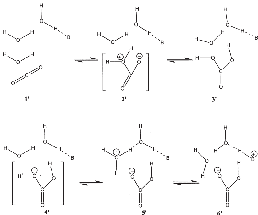
SCHEME 8. Spontaneous \text{CO}_2 uptake and dehydration reaction.
