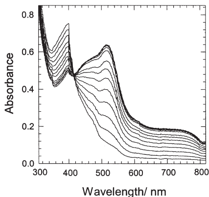
FIG. 16. GO-catalyzed reduction of \text{Os}^{\text{III}} into \text{Os}^{\text{II}} by D-glucose accompanied by a strong absorbance change; [\text{GO}] 1.7 \times 10^{-8} \text{ M} , [\text{D-glucose}] 0.05 \text{ M} , [\text{OsCl}_2(\text{phen})_2^+] 1 \times 10^{-4} \text{ M} , 0.01 \text{ M} phosphate, \text{pH } 6.7 , 25^\circ \text{C} , time intervals 2 min. From Ref. (181).
