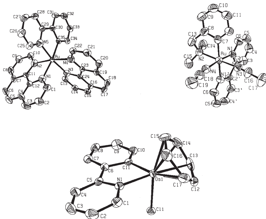
FIG. 21. Crystal structures of cyclometalated \text{Ru}^{\text{II}} and \text{Os}^{\text{II}} complexes [\text{Ru}(\text{phpy})(\text{phen})_2]\text{PF}_6 , [\text{Ru}(\text{dmmba})(\text{bpy})(\text{MeCN})_2]\text{PF}_6 (55) and [(\eta^6\text{-C}_6\text{H}_6)\text{Os}(\text{phpy})\text{Cl}] (235). Counter ions of \text{Ru}^{\text{II}} complexes are not shown for clarity.
