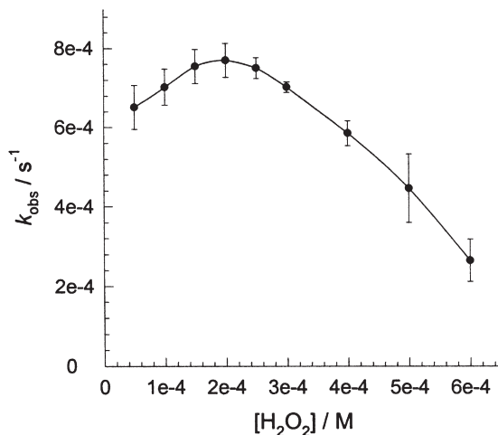
FIG. 20. Dependence of k_{\text{obs}} on \text{H}_2\text{O}_2 concentration for the HRP-catalyzed oxidation of [\text{Ru}(\text{bpy})_2(\text{H}_2\text{O})_2]^{2+} at 25 °C, pH 6.7. From Ref. (181).
