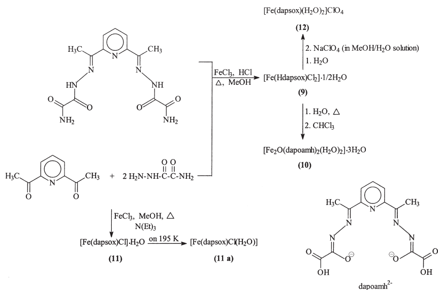
SCHEME 5.
