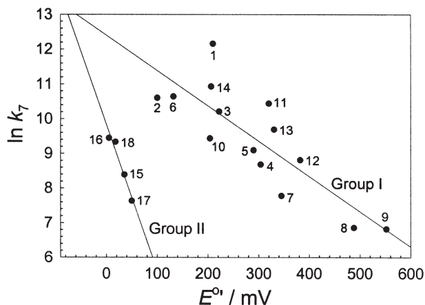
FIG. 9. LFER plot for \ln k_7 (pH 7, 25°C) vs. E^{0'} using the data from Refs. (119,120,130). Numbers correspond to ferrocenes shown in Chart 1.
