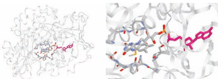
FIG. 1. Subunit of GO from Aspergillus niger with FAD hidden inside the protein globule (left) and a FAD area of GO with amino acid residues in a 8.0 Å vicinity from the N5 atom of FAD (right) (21).
