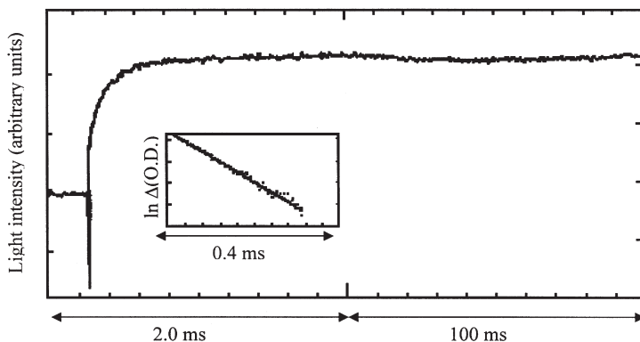
FIG. 1. Computer trace of the time-dependence of the formation of [(\text{NH}_3)_5\text{Co}^{\text{III}}-\text{CH}_2\text{CO}_2]^{+} followed at 300 nm and first order plot (insert). (1 M \text{CH}_3\text{CO}_2\text{Na} , 1 \times 10^{-3} M \text{CoSO}_4 , \sim 20\% \text{NH}_3 , \text{N}_2\text{O} saturated aqueous solution irradiated with a maximum pulse.)
