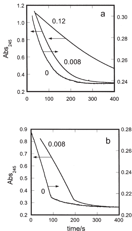
FIG. 10. Effect of methanol and O_2 on the kinetics of Cr_{aq}OO^{2+}/CMe_3CHO reaction in 0.1 M HClO_4 at [CMe_3CHO] = 30 mM, \lambda 245 nm. (a) 0.03 mM Cr_{aq}OO^{2+} , 1 mM O_2 at various concentrations of methanol (0, 0.008, and 0.12 M). (b) Air-free, in the absence of methanol (right ordinate) or in 0.008 M methanol (left ordinate). Reproduced with permission from J. Am. Chem. Soc. 2000 , 122 , 1092–1097. Copyright 2000 American Chemical Society.
