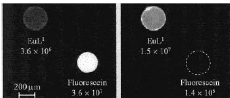
FIG. 9. Microscope luminescence imaging of a model system consisting of oxirane acrylic beads (diameter < 250 \mu\text{m} ) containing [\text{Eu}(\text{HL})]^+ or fluorescein. The left panel shows the prompt fluorescence image and the right panel the TR luminescence image. The figures represent the average luminescence intensities measured for each bead. Reprinted with permission from J. Am. Chem. Soc. 2001 , 123 , 2436–2437. Copyright 2001 American Chemical Society.
