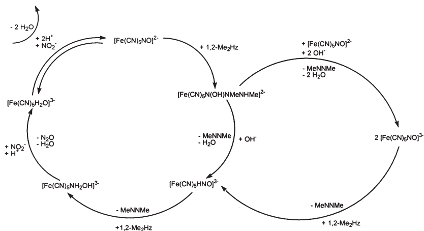
FIG. 15. Catalytic mechanism for the addition of 1,2-Me 2 H 2 to [\text{Fe}(\text{CN})_5\text{NO}]^{2-} in excess of nitrite, showing the participation of [\text{Fe}(\text{CN})_5\text{NO}]^{3-} in an alternative path.
