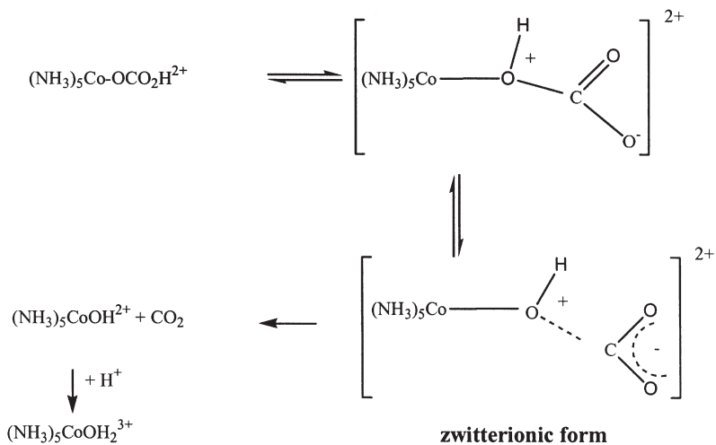
SCHEME 5. Decarboxylation of [(\text{NH}_3)_5\text{CoOCO}_2\text{H}]^{2+} through its zwitterionic form.
