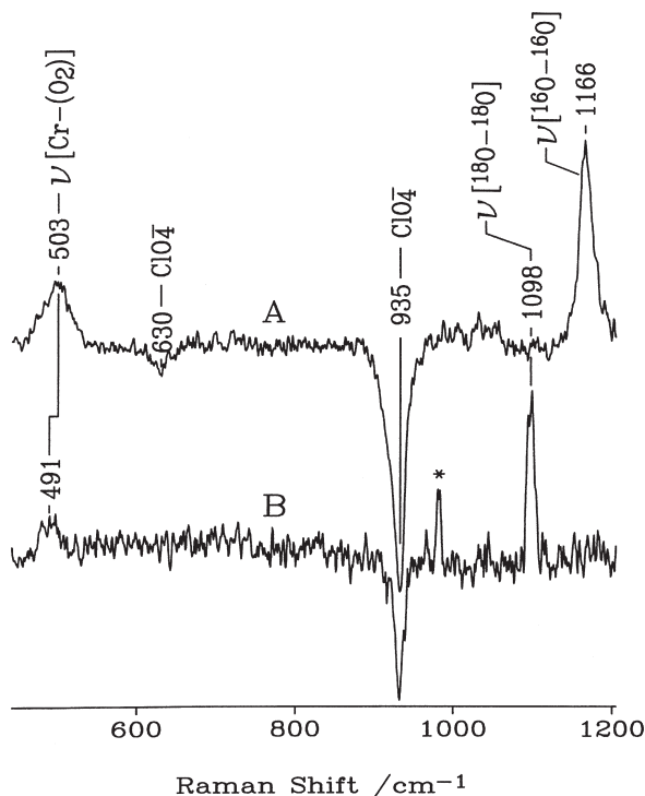
FIG. 2. 245-nm excited resonance Raman spectrum of (A) 0.225 mM \text{Cr}_{\text{aq}}\text{OO}^{2+} and (B) 50 \mu\text{M Cr}_{\text{aq}}^{18}\text{O}^{18}\text{O}^{2+} in 0.02 M \text{HClO}_4 at 0 ^\circ\text{C} . Negative peaks arise from subtraction of the intense \text{HClO}_4 bands at 934 and 629 \text{cm}^{-1} . The asterisk indicates a burned spot on the intensifier of the diode-array detector. Reproduced with permission from J. Am. Chem. Soc. 1995, 117, 6483–6488. Copyright 1995 American Chemical Society.
