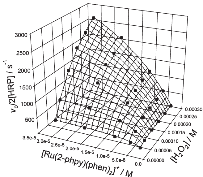
FIG. 22. 3D plot showing steady-state rate of the HRP-catalyzed oxidation of [\text{Ru}(\text{phpy})(\text{phen})_2]^+ by \text{H}_2\text{O}_2 against [\text{H}_2\text{O}_2] and [\text{Ru}^{\text{II}}] at [\text{HRP}] 5 \times 10^{-11} , pH 6.7, 2% MeOH, 25 °C. From Ref. (55).
