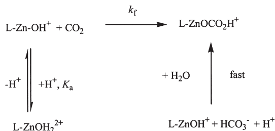
SCHEME 3. \text{CO}_2 uptake reaction of [\text{LZnOH}]^{(n-1)+} species; \text{L} = [12]\text{aneN}_3 .
