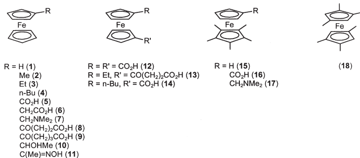
CHART 1. Ferrocenes studied as substrates of HRP (120).
