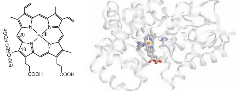
SCHEME 3. Structures of hemin, the iron(III) complex of protoporphyrin IX, and recombinant HRP isoenzyme C (29).
