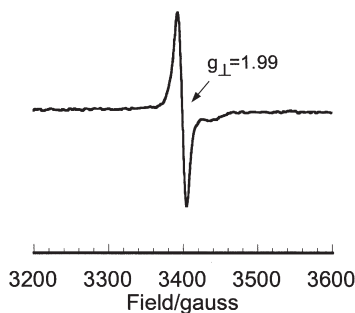
FIG. 5. First derivative ESR spectrum of L^1Cr(V) ( L^1 = 14\text{-aneN}_4 ) in 1:1 H_2O /propylene glycol glass at 120 K. Reproduced with permission from J. Am. Chem. Soc. 1996 , 118 , 10325–10326. Copyright 1996 American Chemical Society.
