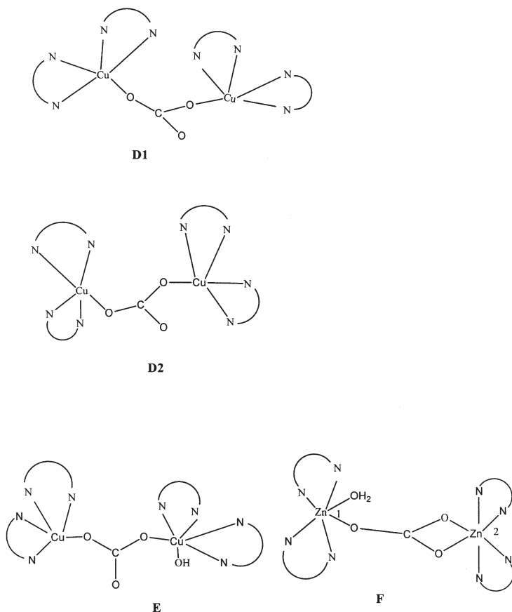
FIG. 6. Binuclear carbonato bridged complexes. N-N=phen ( D and E ); N-N=bpy ( F ).
