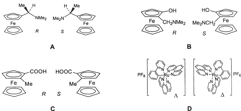
CHART 2. Examples of chiral complexes studied in redox reactions with GO, HRP, and cytochrome c peroxidase.
