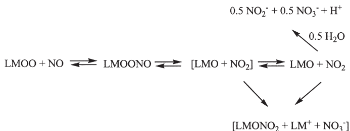
SCHEME 9.
