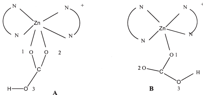
FIG. 4. [(phen) 2 ZnHCO 3 ] + . A – chelated; B – monodentate bicarbonato.
