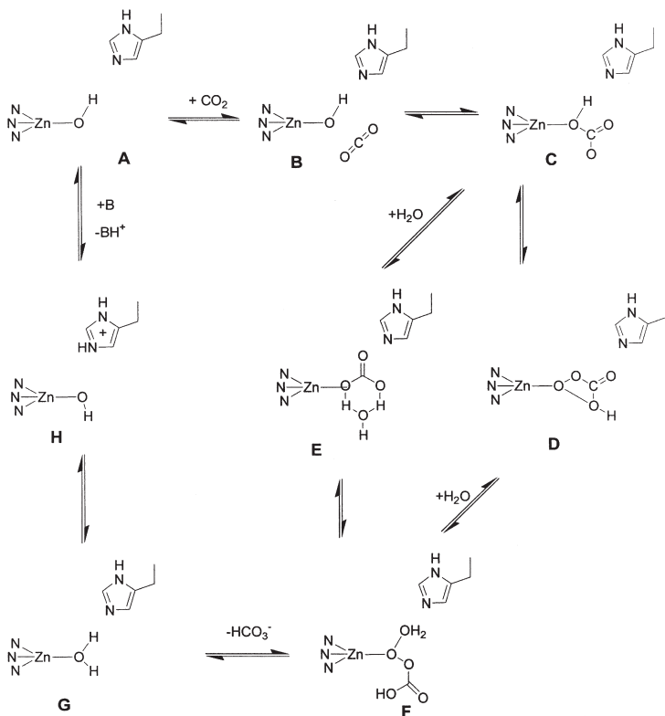
SCHEME 6. Proposed CO_2 hydration mechanism for HCA II ( \alpha -CA).
