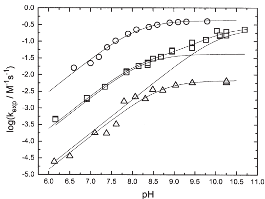
FIG. 12. Dependence of \log k_{\text{exp}} on pH for the reaction of [\text{Fe}(\text{CN})_5\text{NO}]^{2-} with hydrazines. Upper curve: Hz; intermediate curve: MeHz; lower curve: 1,1-Me 2 H z . T=25.0^\circ\text{C} , I=0.1\text{ M} . For MeHz, the broken lines represent the individual contributions of each term in the rate equation (62).
