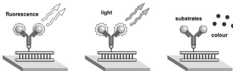
FIG. 28. Synthesis of labeled DNA probes. A: Labeled DNA can be generated using different enzymes (Klenow fragment of DNA polymerase or a terminal transferase) to incorporate labeled nucleotides into specific DNA sequences. Probes can be labeled using radioactive nucleotides or nucleotides labeled with an immunogenic molecule such as biotin. B: The labeled probe is then hybridized to the target nucleic acid, which is either bound to a membrane or in a tissue section or cell. An antibody is then used to detect the non-radioactively-labeled probe. C: The antibody may be conjugated to a fluorescent or chemiluminescent dye, or an enzyme that produces a color reaction. The target nucleic acid is thus visualized.
