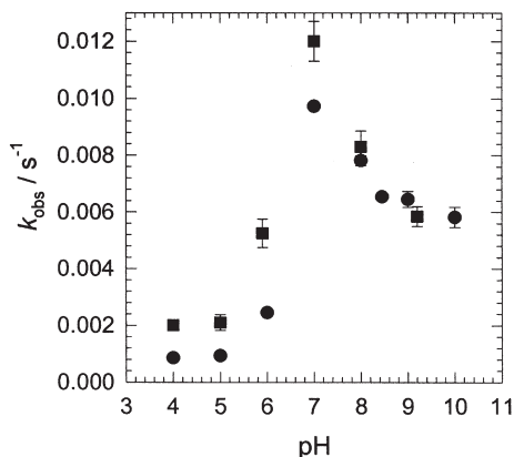
FIG. 17. pH-dependence of k_{\text{obs}} for the GO-catalyzed oxidation of [\text{Os}(\text{phen})_2\text{Cl}_2]^+ by D-glucose in 0.01 \text{ M} \text{NaClO}_4 (■) and 0.01 \text{ M} phosphate (●); 25^\circ \text{C} , [\text{Triton X-100}] 2\% , [\text{GO}] 1.5 \times 10^{-7} \text{ M} , [\text{D-glucose}] 0.05 \text{ M} . From Ref. (181).
