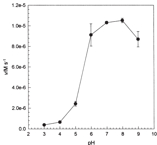
FIG. 4. pH profile for the steady-state rate of GO-catalyzed reduction of \text{Fc}^+ \text{PF}_6^- at [\text{Fc}^+] 0.002 \text{ M} , [\text{D-glucose}] 0.05 \text{ M} , [\text{GO}] 2 \times 10^{-7} \text{ M} , 25^\circ \text{C} , phosphate buffer, [\text{Triton X-100}] 2\% \text{ (v/v)} ; from Ref. (79).
