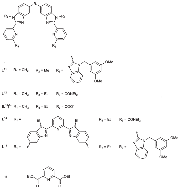
SCHEME 2. Selected Bünzli/Piguët ligands.
