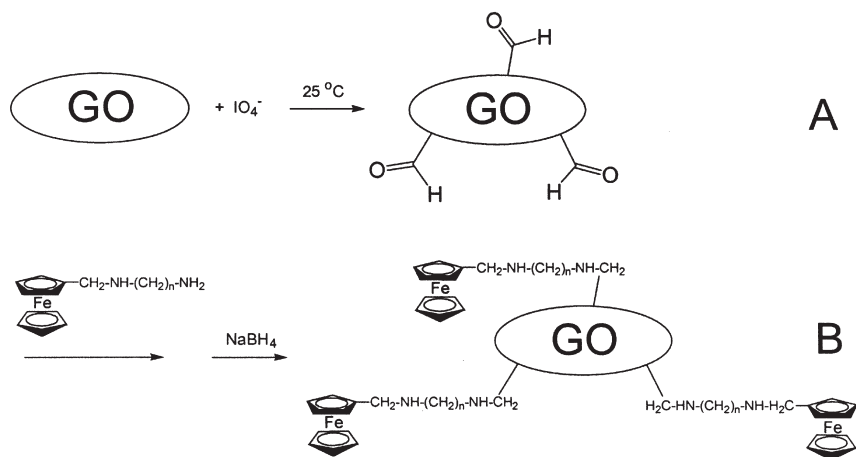
SCHEME 7. Preparation of GO modified by peripherally bound ferrocenes. From Ref. (106).
