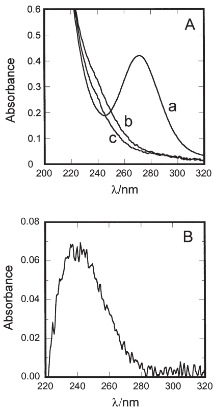
FIG. 14. (A) Spectral changes observed upon mixing 42 \mu\text{M L}^2(\text{H}_2\text{O})\text{RhOO}^{2+} (spectrum a ) with 0.1 \text{ mM NO} in 0.015 \text{ M HClO}_4 . Spectrum b was recorded immediately after mixing, and spectrum c 200 min later. (B) Difference spectrum ( b-c ) of the intermediate \text{L}^2(\text{H}_2\text{O})\text{Rh}(\text{NO}_3)^{2+} . Reproduced with permission from J. Am. Chem. Soc. 2002 , 124 , 1698–1703. Copyright 2002 American Chemical Society.
