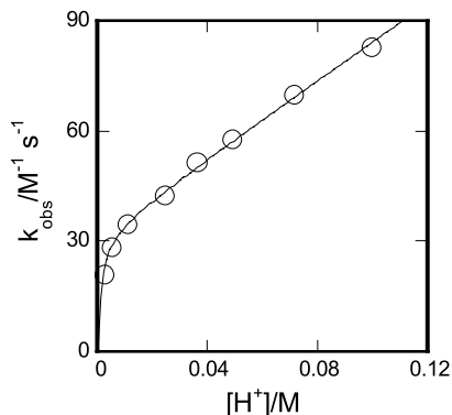
FIG. 15. Plot of k_{\text{obs}} vs. [\text{H}^+] for the reaction between \text{L}^2(\text{H}_2\text{O})\text{RhOO}^{2+} and \text{HNO}_2 . The solid line is the fit to Eq. (47). Reproduced with permission from Inorg. Chem. 2002 , 41 , 901–905. Copyright 2002 American Chemical Society.
