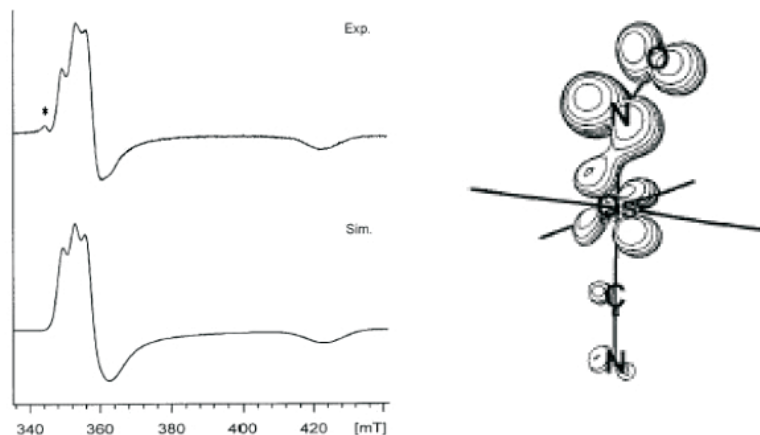
FIG. 1. (Left) Experimental and simulated EPR spectra of electrogenerated [\text{Os}(\text{CN})_5\text{NO}]^{3-} in AcN/0.1 M \text{Bu}_4\text{NPF}_6 , at 3.5 K. (The asterisk denotes a low-field impurity) (Right) Spin density distribution within [\text{Os}(\text{CN})_5\text{NO}]^{3-} .
