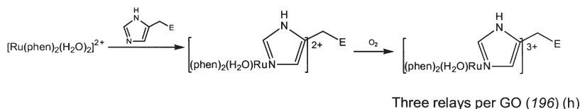
SCHEME 14. Continued.
