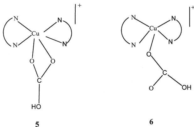
FIG. 2. [\text{Cu}(\text{phen})_2(\text{OCO}_2\text{H})]^+ : N-N = 1,10-phenanthroline. 5 – Lipscomb structure; 6 – Lindskog structure.
