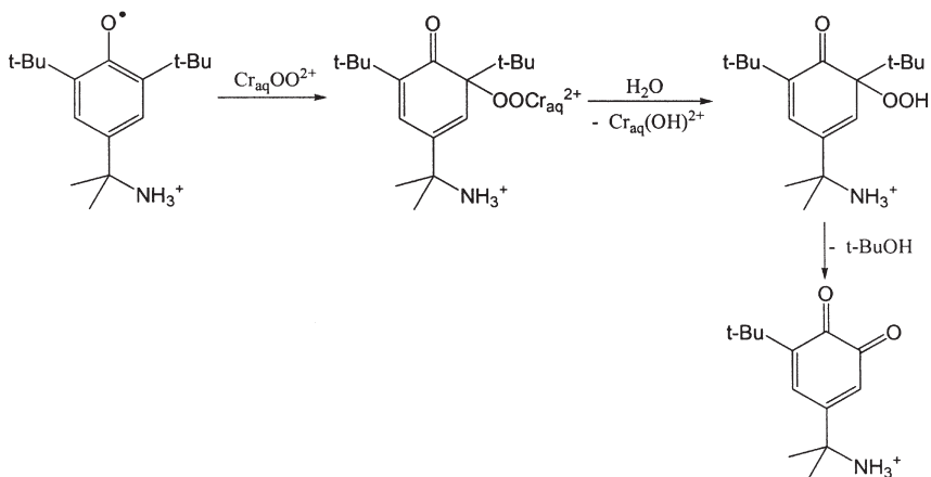
SCHEME 5.
