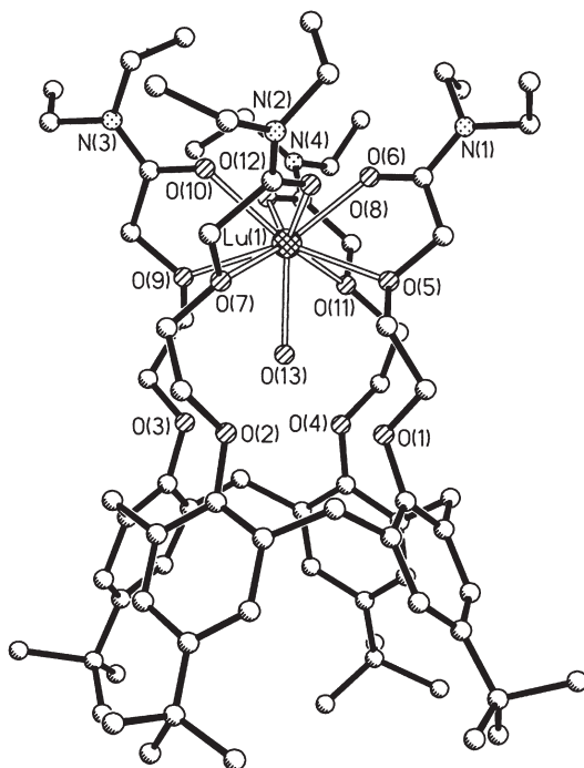
FIG. 13. Molecular structure of [\text{Lu}(\text{L}^{49})(\text{H}_2\text{O})]^{3+} . This figure was generated from data obtained from the Cambridge Crystallographic Data Centre as published originally in Ref. (83).
