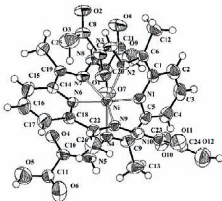
FIG. 4. The structure of complex cation [\text{Ni}(\text{H}_2\text{dapoamh})_2]^{2+} (11).
