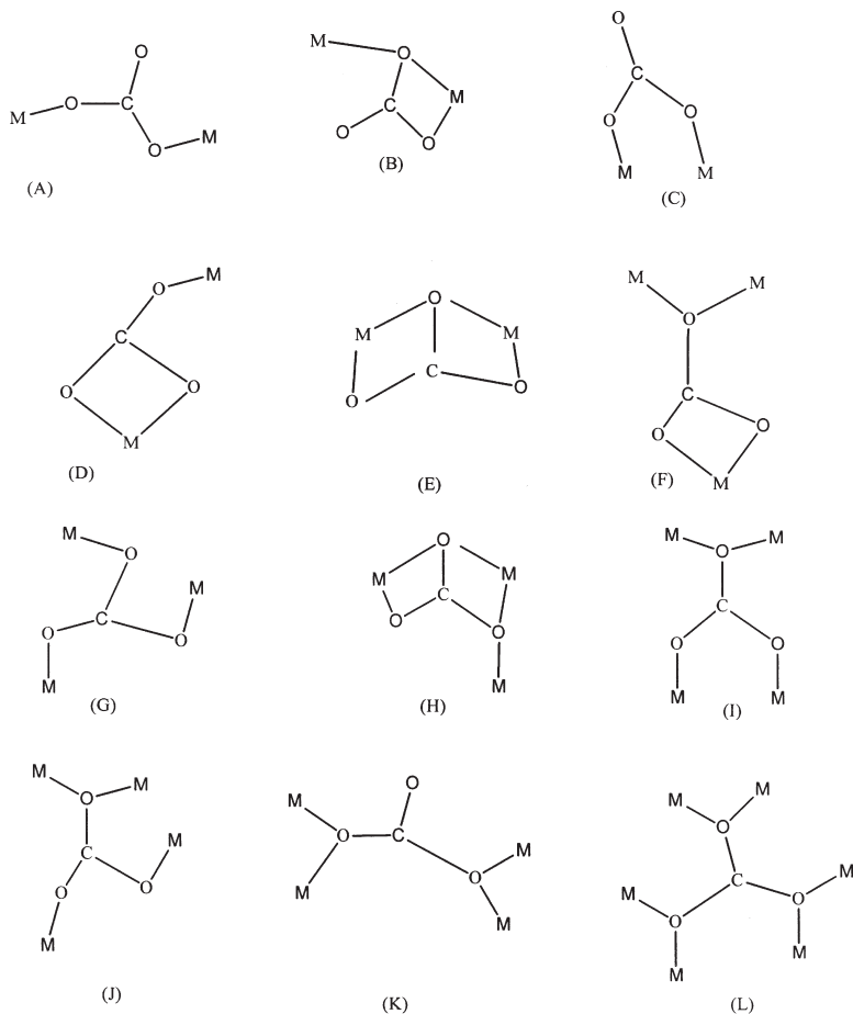
CHART 1. Different coordination modes of carbonate in metal carbonates.
