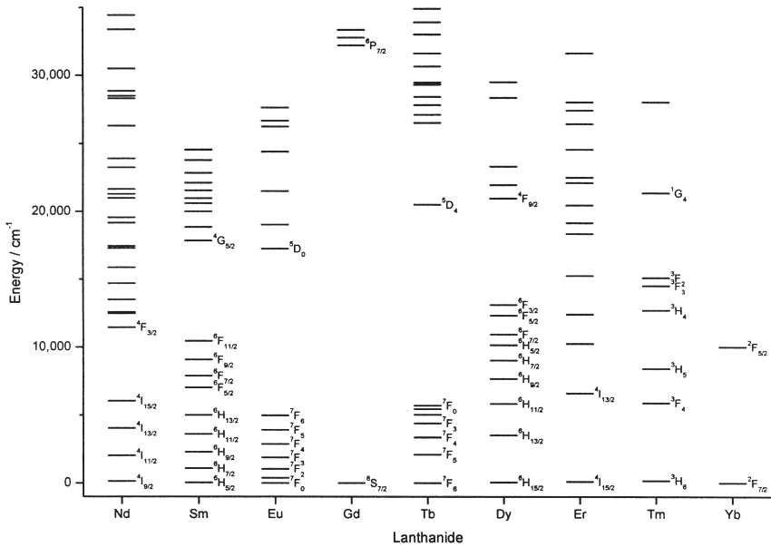
FIG. 1. Energy levels of selected lanthanide(III) ions (199).
