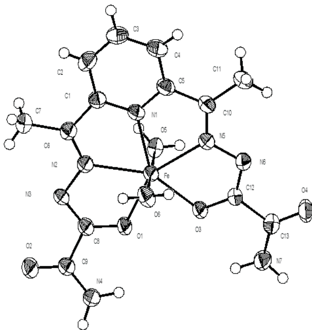
FIG. 6. The structure of complex cation [\text{Fe}(\text{dapsox})(\text{H}_2\text{O})_2]^+ ( 12 ).
