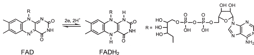
SCHEME 2. Structures of oxidized (FAD) and reduced (FADH 2 ) forms of flavin adenine dinucleotide.
