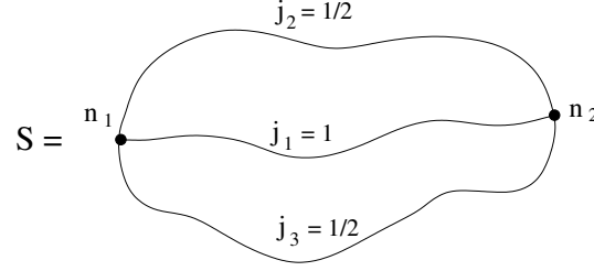
Figure 1.2: A simple spin network.
