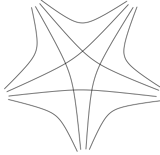
Figure 9.8: The structure of the vertex of the fat 5-valent graphs generated by the Feynman expansion.
