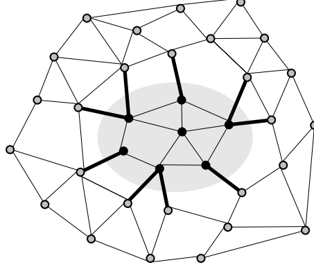
Figure 6.9: Regions and surfaces defined on an s -knot: the set of the black nodes define a “region” of space; the set of the black links define the “surface” surrounding this region.
