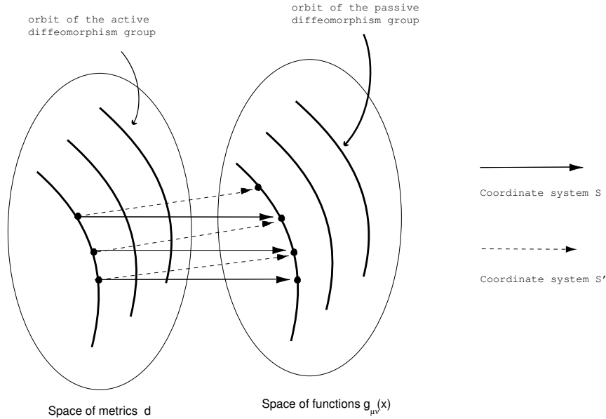
Figure 2.2: Active and passive diffeomorphisms.
