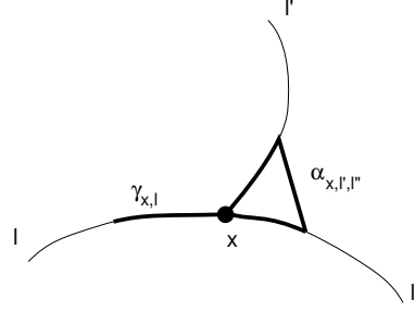
Figure 7.1: The path \gamma_{x,l} and the loop \alpha_{x,l',l''} at a triavalent node in the point x .
