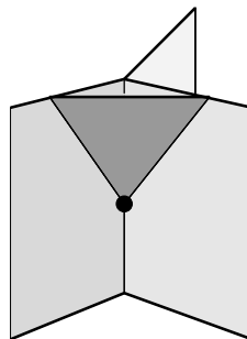
Figure 9.3: A vertex of a spinfoam.
