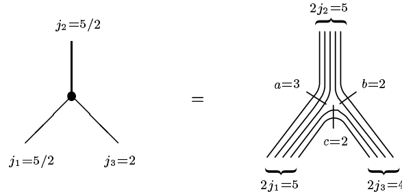
Figure A.1: Clebsh-Gordon condition.
