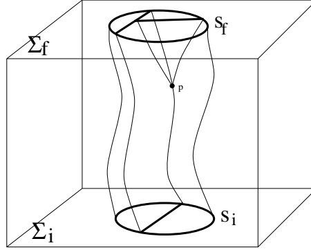
Figure 9.4: A spin network with one vertex.
