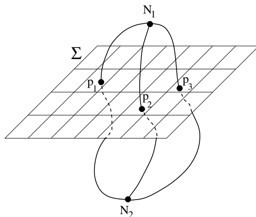
Figure 6.5: A simple spin network S intersecting the surface \mathcal{S} .
