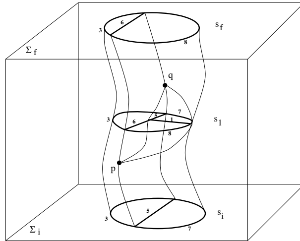
Figure 9.5: A spin network with two vertices.
