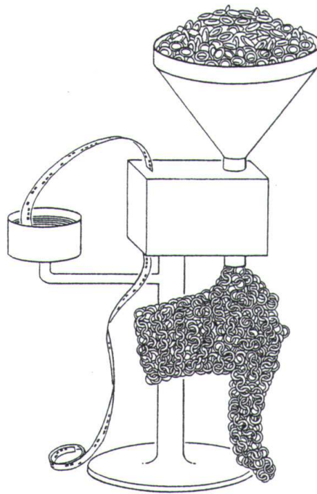
Figure B.1: The weave, in Wheeler's vision.
