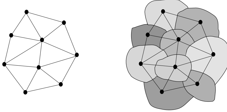
Figure 6.8: The graph of an abstract spinfoam and the ensemble of “chunks of space”, or quanta of volume, it represents. Chunks are adjacent when the corresponding nodes are linked. Each link cuts one elementary surface separating two chunks.
