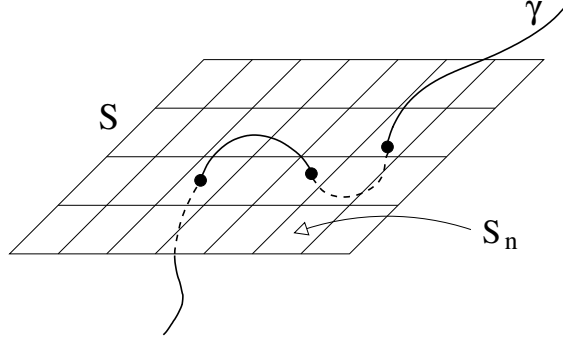
Figure 6.4: A partition of \mathcal{S} .
