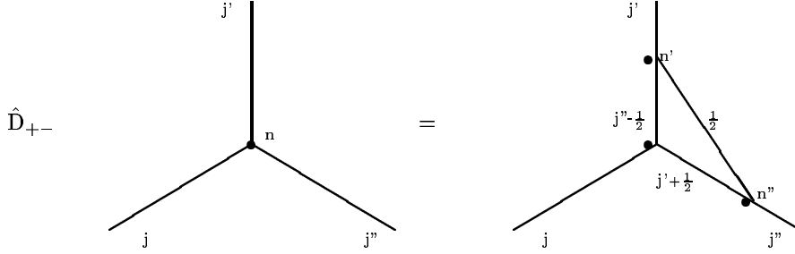
Figure 7.2: Action of D_{n,l',l'',r,\epsilon',\epsilon''} .
