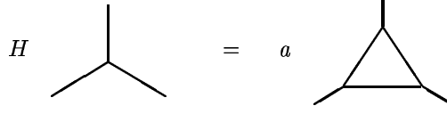
Figure 9.1: Scheme of the action of H on a node of a spin network.
