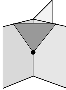
Figure 1.5: The vertex of a spinfoam.
