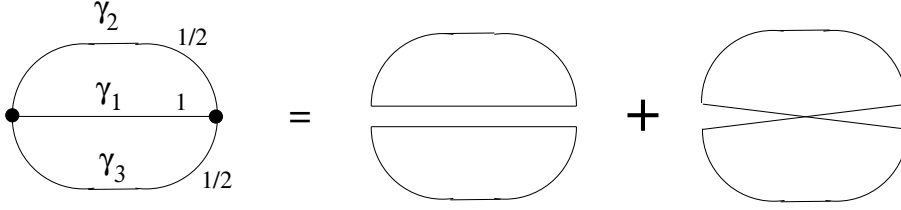
Figure 6.2: Decomposition of a spin network state into loop states.
