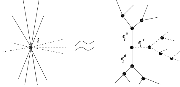
Figure 6.7: Trivalent expansion of an n -valent vertex. The dashed lines indicate the lines tangent to the surface.
