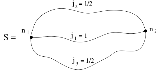
Figure 6.1: A simple spin network with two trivalent nodes.
