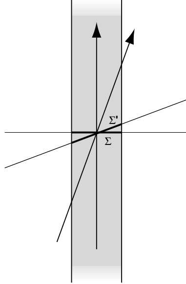
Figure 8.1: The grey region represents the world history of an object. The two arrows represent the worldlines of two observers. The bold segments \Sigma and \Sigma' are the intersections between the object world history and the observers' equal time surfaces. Two observers in relative motion measuring the length of the same object measure the gravitational field on these two distinct surfaces. The gravitational field on \Sigma does not commute with the gravitational field on \Sigma' . Hence the two lengths do not commute.
