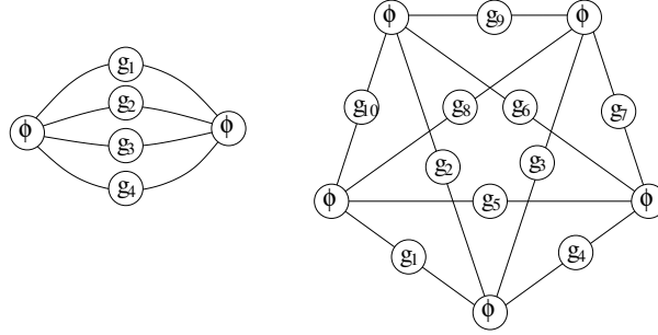
Figure 9.6: The structure of the kinetic and potential terms in the action.
