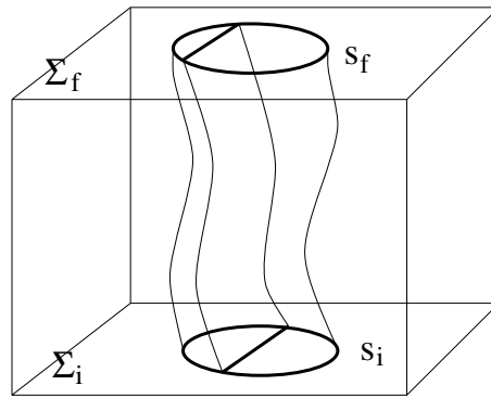
Figure 9.2: The worldsheet of a spin network.
