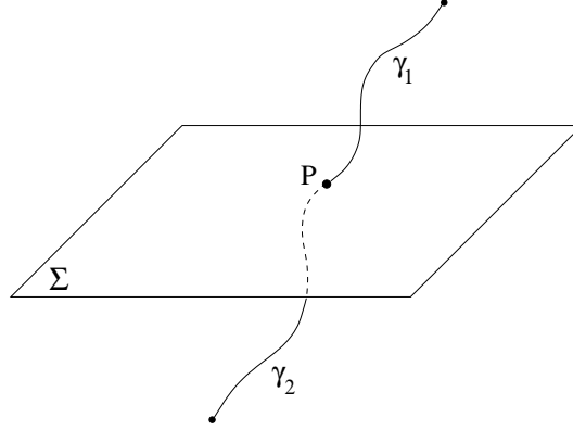
Figure 6.3: A curve that intersects the surface in an individual point.
