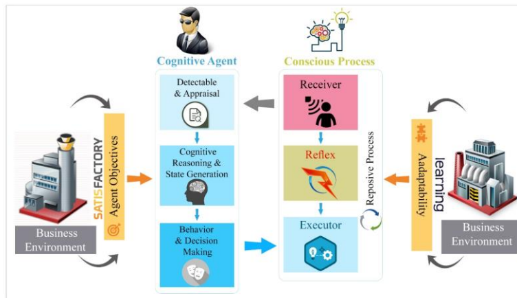
FIGURE 3. Agent model [16]
