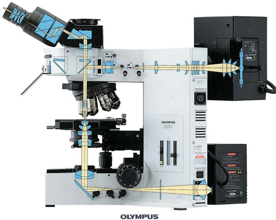
Color Plate 4-1. Optical path in the Olympus BX60 upright microscope. The microscope is fitted with a transilluminator (bottom) and epi-illuminator (top) and has infinity-corrected optics. Lenses, filters, and prisms are light blue. Light passing through the objective lens emerges and propagates as a parallel beam of infinite focus, which is collected by an internal tube lens (Telan lens) as an aberration-free image in the real intermediate image plane. The Telan lens is located where the black trinocular headpiece joins the white microscope body. The infinity space between objective and Telan lens allows insertion of multiple optical devices (fluorescence filter sets, waveplate retarders, DIC prisms, analyzer, and others) without altering the magnification of the image. This color plate was provided by Olympus America, Inc.
