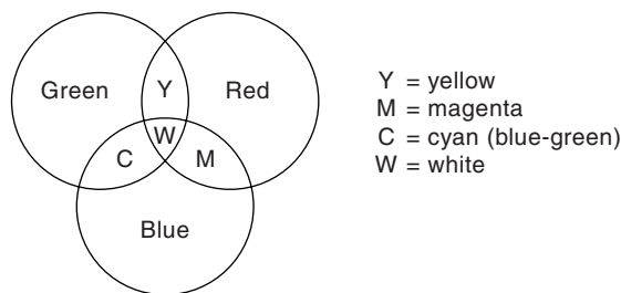
Figure 2-9 Addition colors of the red-green-blue tricolor system. This color display can be produced by projecting the colors of RGB color filters with three separate slide projectors on a screen as described in the text.
