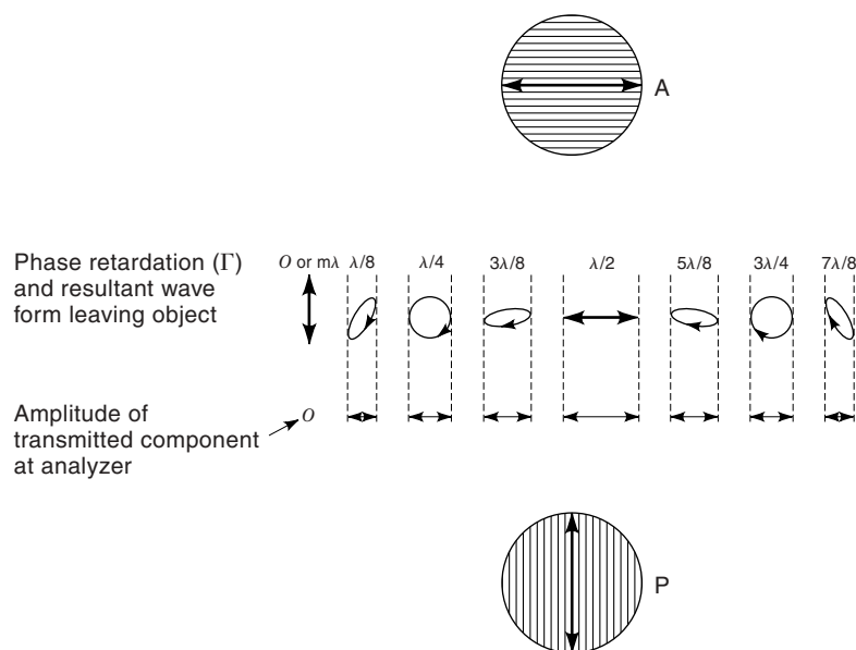
Figure 8-12 Effect of relative phase shift between O and E rays on the waveform of polarized light. Waves resulting from the combination of superimposed O and E rays have elliptical, spherical, or planar waveforms, depending on the amount of relative phase shift between the two rays. The orientations of the transmission axes of the polarizer and analyzer are indicated. The amplitudes of the components of vibration passing the analyzer are also shown.
