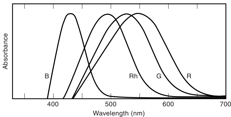
Figure 2-8 Absorption difference spectra of the four human visual pigments. The four pigment proteins were cloned, purified, and characterized with respect to their absorption spectra in vitro. Photobleaching difference spectra were obtained by subtracting an absorption spectrum measured after light exposure from one measured prior to light exposure. The pigments show maxima in the expected red, green, and blue regions of the visual spectrum. The values are close to those measured for rod and cone cells in vivo and confirm Maxwell’s theory for RGB-based color vision over a century ago. (Courtesy of Jeremy Nathans, Johns Hopkins University.)
