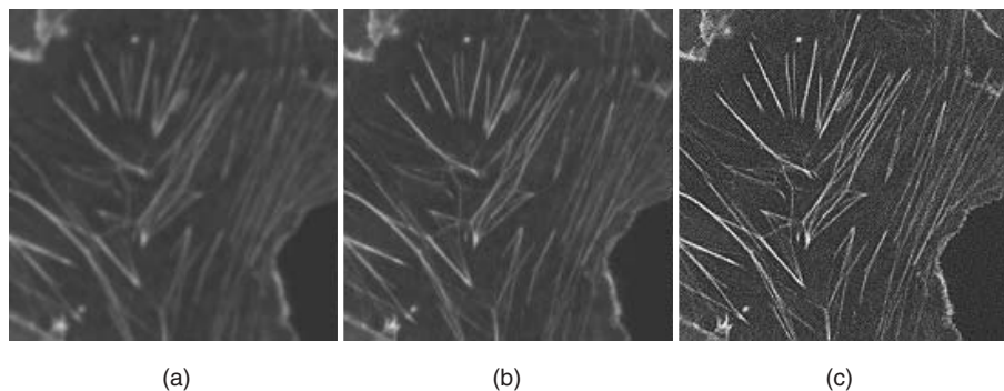
Blurring kernel
