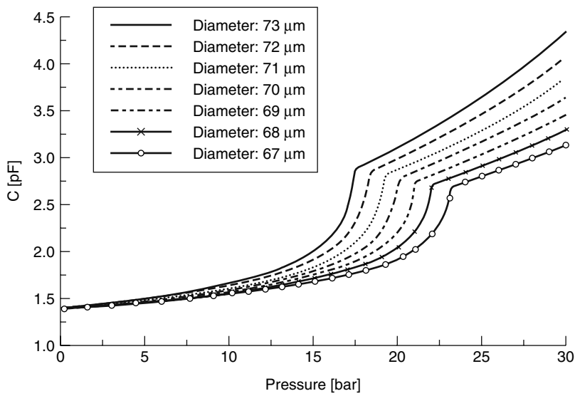
Figure 8.15 Parametric Saber simulations for the variation of the diameter of the pressure element. The plate thickness is fixed at 1.7 μm
