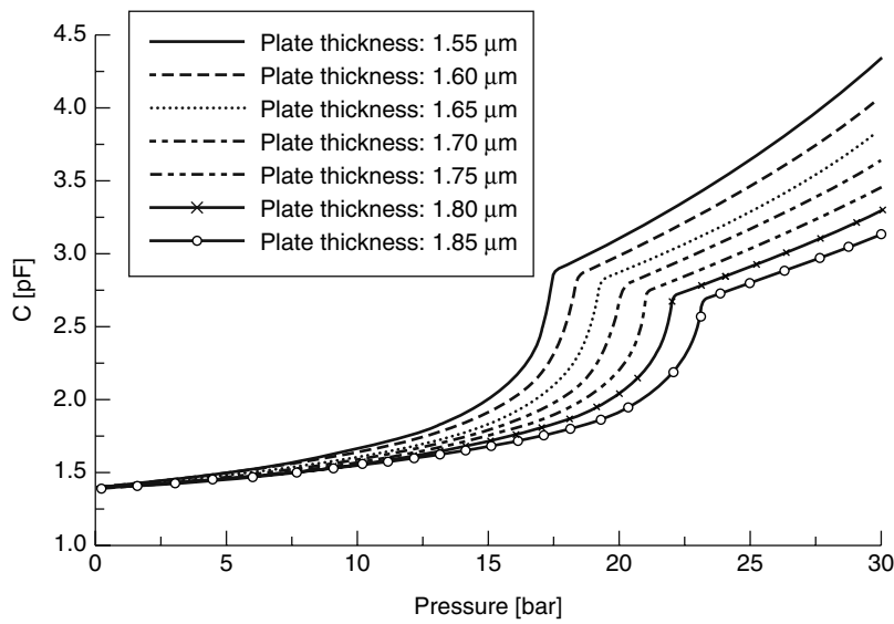
Figure 8.16 Parametric Saber simulations for the variation of the plate thickness of the pressure element. The diameter is fixed at 70 μm
