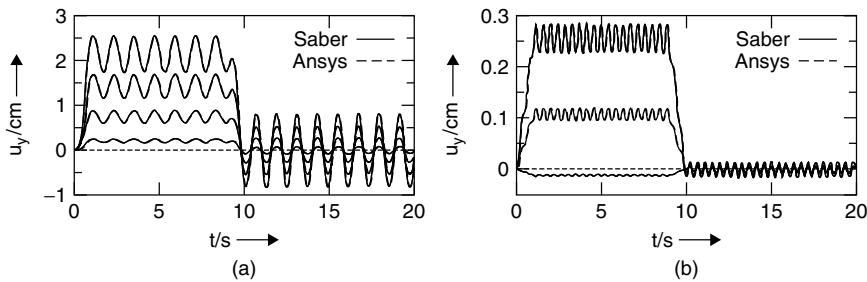
Figure 6.11 Simulation results for the deflection at x = 0.25l, 0.51, 0.75l and 1.0l of a cantilever beam with (a) and without (b) an additional support
