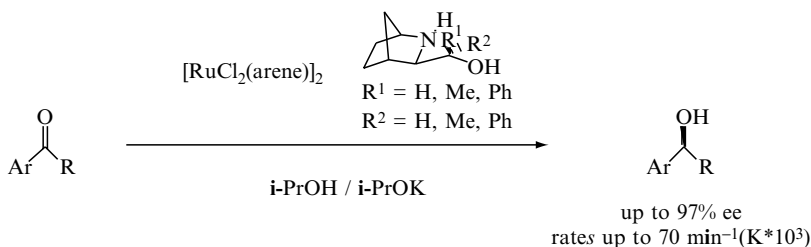
Figure 9.2 Transfer hydrogenation of ketones catalyzed by Ru(II)(2-azanobornyl-methanol) complexes.
