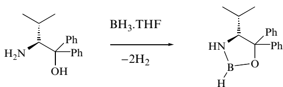
Figure 11.1 Complexation of borane with valinol [1] .
