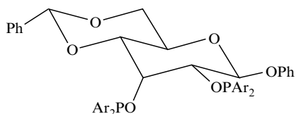
(60) Ar = 3,5-bis-trifluorophenyl
