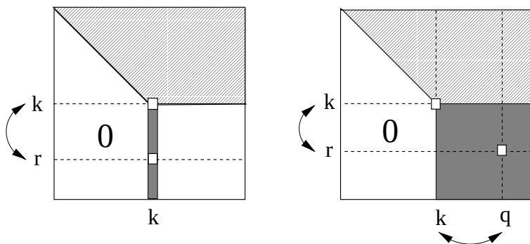
FIGURE 3.2. Partial pivoting by row (left) or complete pivoting (right). Shaded areas of the matrix are those involved in the searching for the pivotal entry
