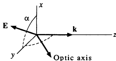
Fig. 1.2. Coordinates used to describe double refraction: The incident wave vector \mathbf{k} is along the z -axis; the electric vector \mathbf{E} is in plane xy ; and the optic axis of the crystal is in plane yz .
