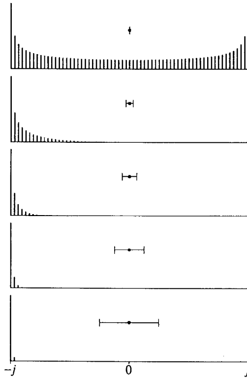
Fig. 12.7. Expected probability distributions for a second measurement of J_z , after one more rotation by \pi/2 . The results depend on the \Delta q of the meter which performed the first measurement. From top to bottom, this \Delta q (shown as a horizontal error bar) is 0, 1, 2, 4, and 8. Different vertical scales are used in the various diagrams, for better visibility. In each diagram, the sum of lengths of the vertical bars is 1, by definition.
