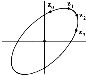
Fig. 11.1. An elliptic fixed point \mathbf{r}_0 is located at the origin of a 2-dimensional surface of section. Consecutive points of a neighboring orbit, \mathbf{r}_0 + \epsilon \mathbf{z}_k , lie on an ellipse.
