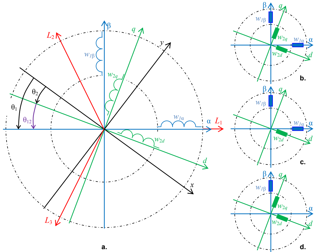
Fig. 4.1 Park's model of a motor
